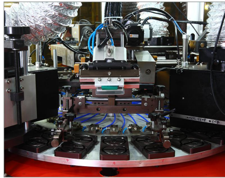
Printing Station
