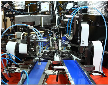
In-feed Conveyor
