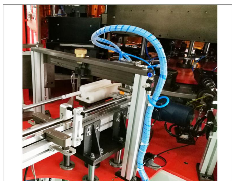
In-feed Conveyor
