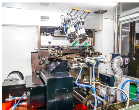
Printing Station
